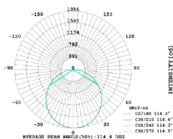
LUMINOUS INTENSITY DISTRIBUTION
